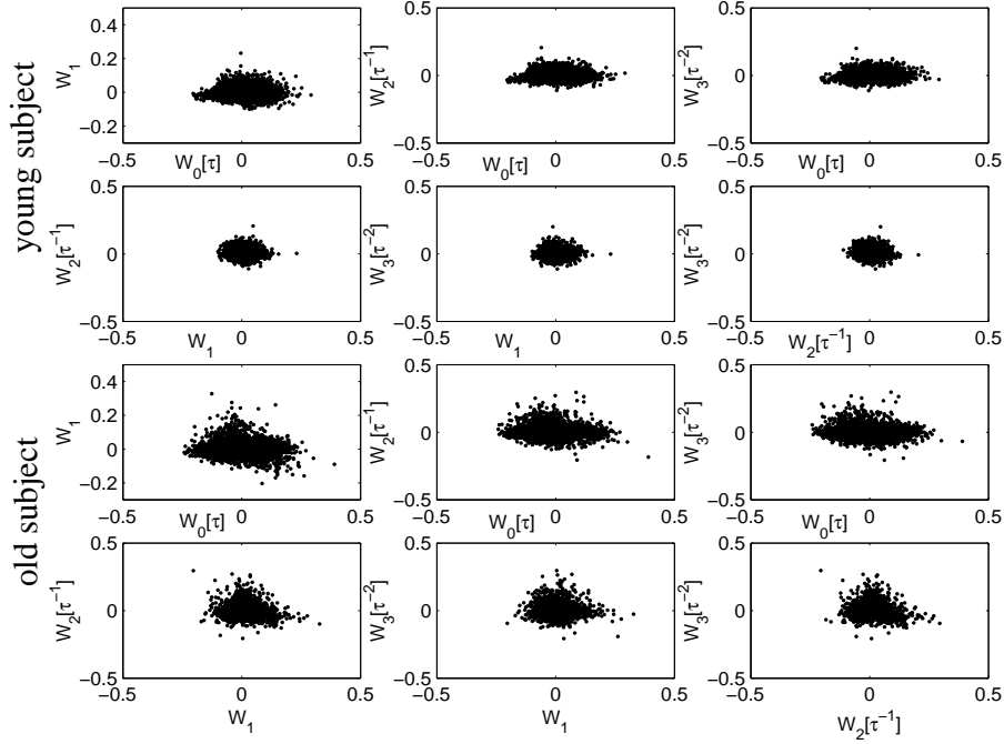
Figure 2: The phase portraits of variability of an R-R interval on six plane projections of various combinations W_i, W_j for young and elderly people. The phase clouds of the young man are more compressed towards the center of coordinates system. Around the centralized nucleus of the phase clouds for the elderly person, separate points are scattered. The interval of their disorder 2-3 times exceeds the areas of disorder of the phase points for the young man.
